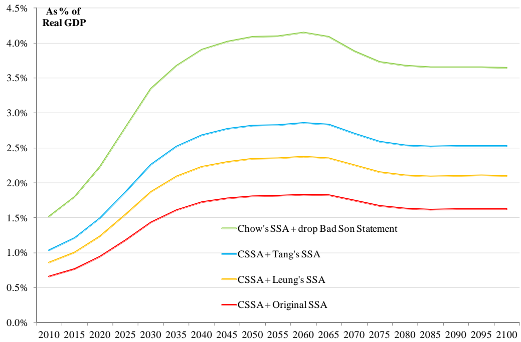
Figure 2: Comparisons of Old Age (65+) Social Security Expenditure as Percentage of Real GDP, 2010-2100
